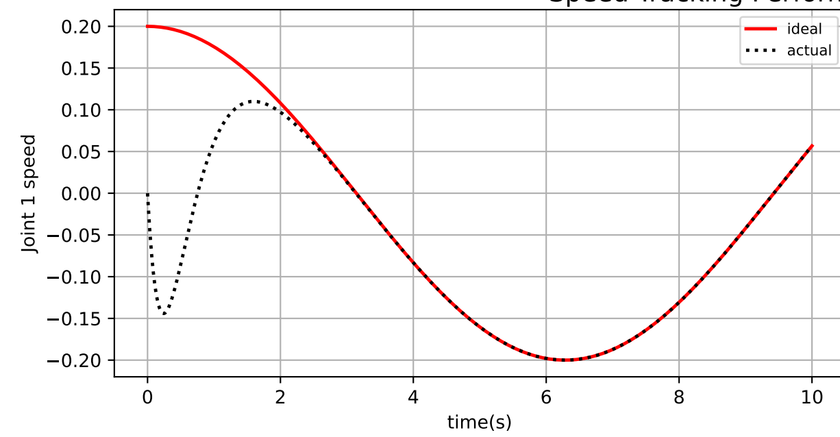
Speed Tracking Performance (S=2, S1=2, m=5)
